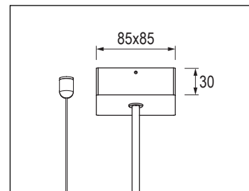
Square Canopy
