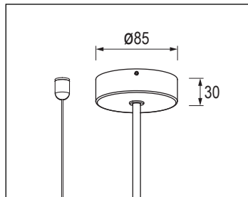
Round Canopy
