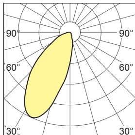
Asymmetric
