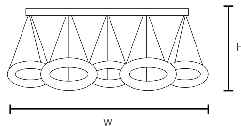
AD-MD-C-5A: L 1800 x W 500 x H 1500
