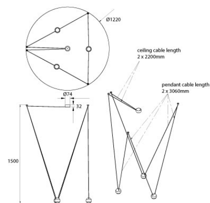
AD-P 77-3 Ø 74 x 1500 *units in mm
